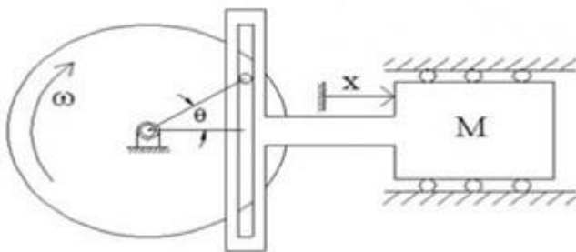
Fig. 5 Scotch Yoke Mechanism
