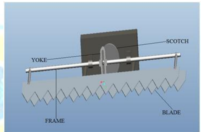
Fig. 6 Harvester Design
