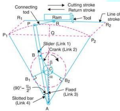
Fig. 23 Scotch Yoke Mechanism
