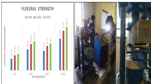
Fig. 3: Flexural Strength of Beam
