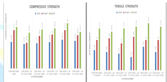
Fig. 2: Compressive strength & Tensile strength of Concrete
