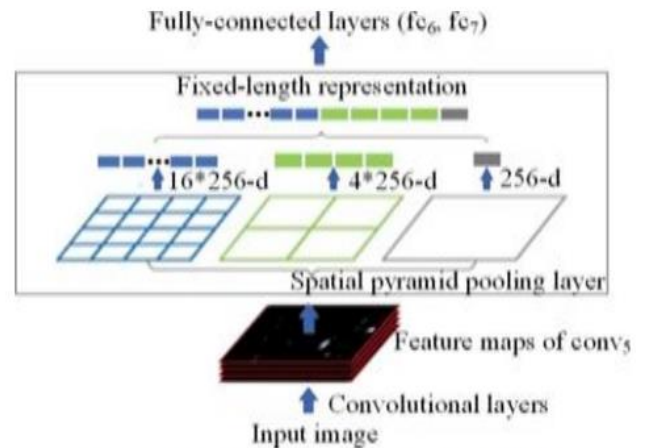
Fig.2 : SPP-Net Space Pyramid Structure
