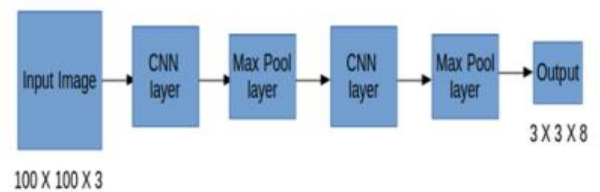
Fig.5 : Yolo Flow Chart
