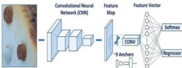
Fig.3 : RPN Network Structure
