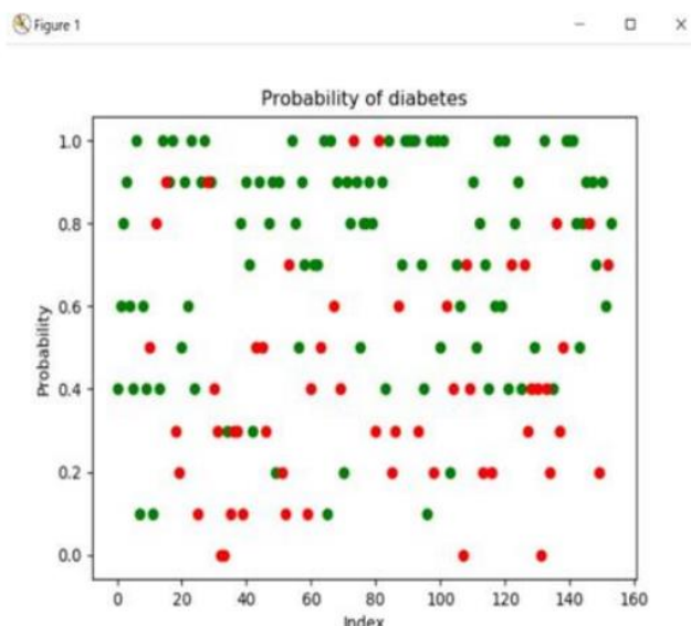
Figure 3: Probability Chart
