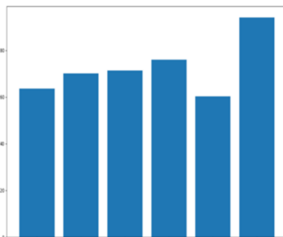
Figure 6: Accuracy results
