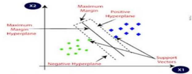
Fig 3. Classes of Support Vector Machine –SVM [23]
