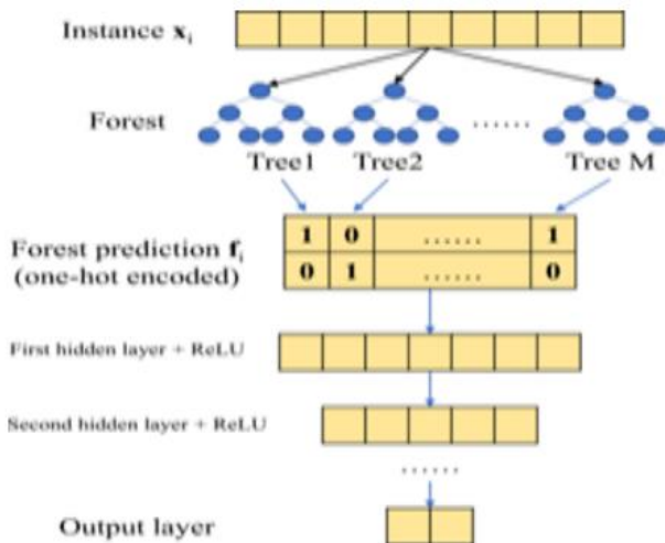
Fig 2. Hierarchy of Random Forest [6]
