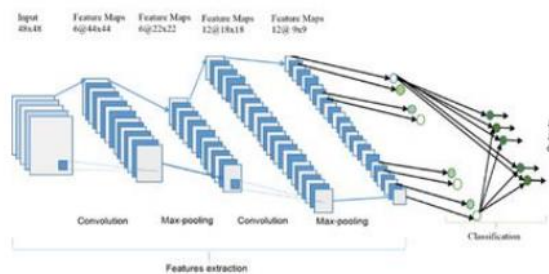
Fig 1 . Architecture of Convolutional neural network – CNN [22]
