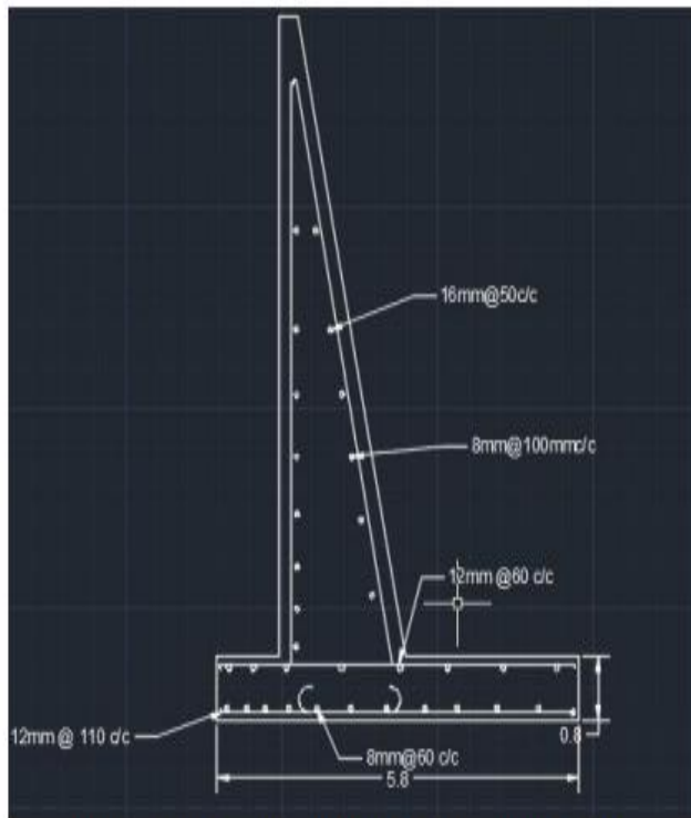
Fig 1 Reinforcement Detail In Retaining Wall
