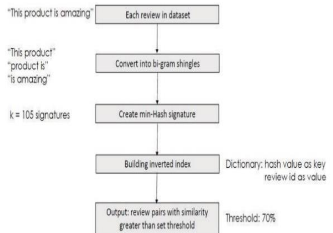
Figure 1. Overall process of bi-gram algorithm
