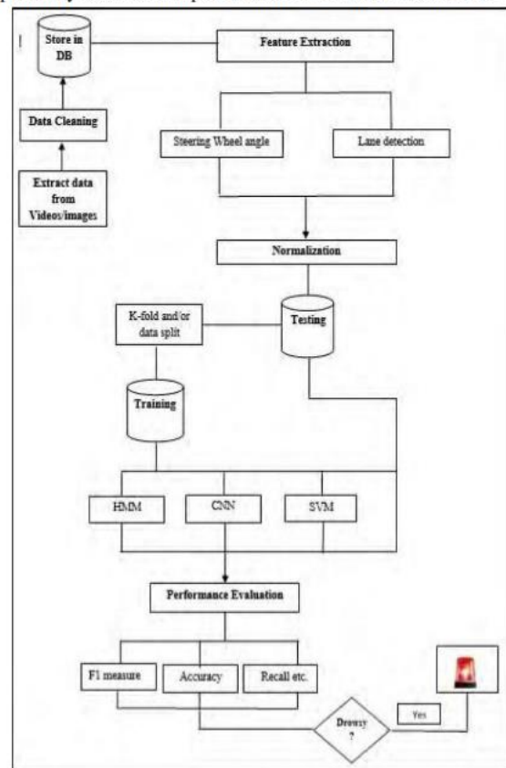
FIGURE 2. A general framework of vehicular pattern-based techniques.
