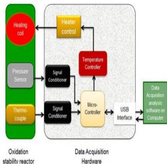
Figure 2.2: Automation of Control and Monitoring system
