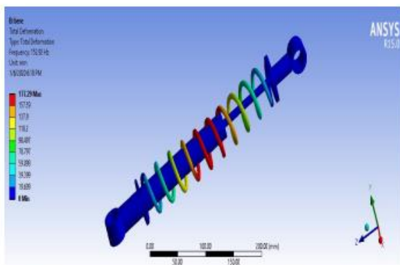
Fig 2: First mode shape of Berelium Copper
