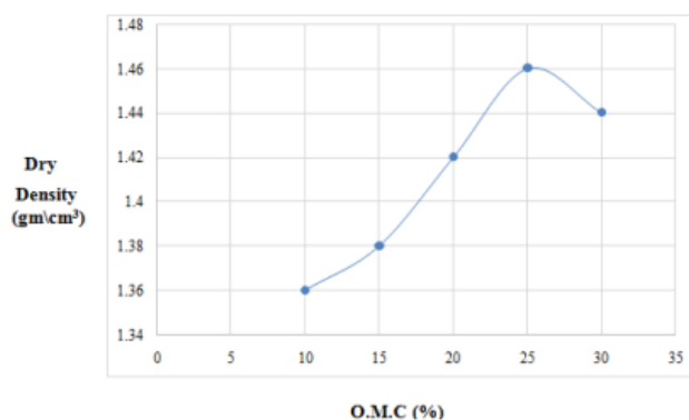
Graph: 3.1. Black cotton soil
