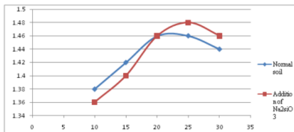
Graph 3.3: Black cotton soil
