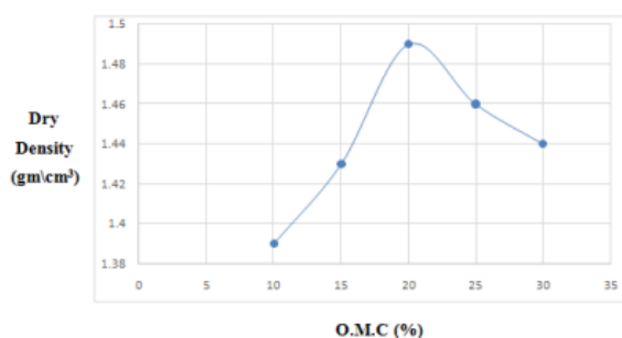
Graph: 3.1. Red soil
