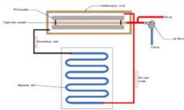
Fig no. 1 solar heating system
