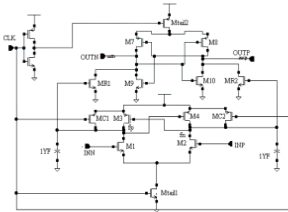
Fig 5. Schematic of the existing Double tail comparator with static power consumption
