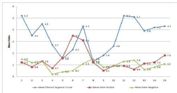
Figure 5. Comparison of MFSC, MFP and MFN
