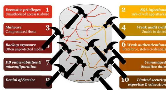
Figure 1. Database Threats
