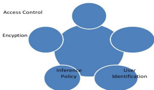
Figure 2. Control Methods
