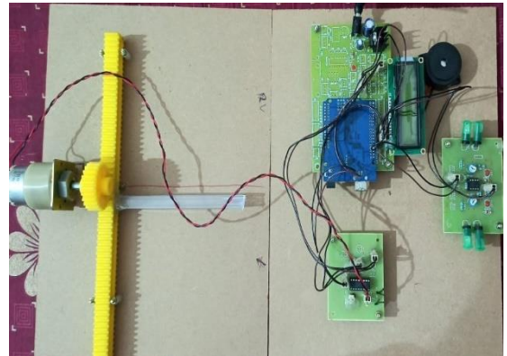
FIGURE 5: Functional setup of road divider circuit
