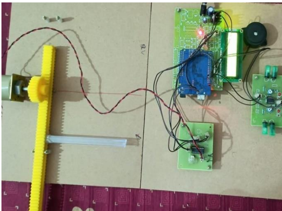
FIGURE 8: Divider moves towards left.
