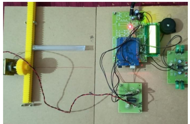
FIGURE 10: divider moves towards right
